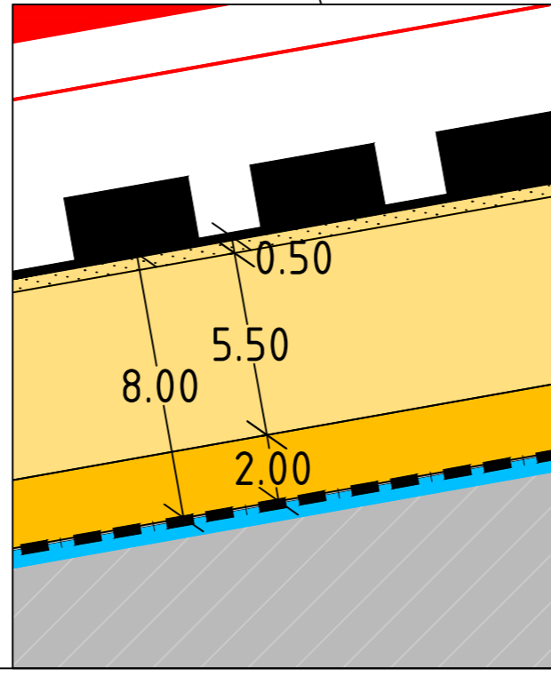
Detailplan M 1 : 200
